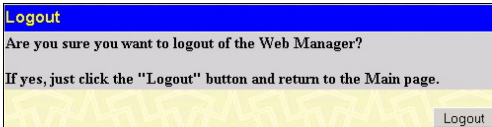
Figure 10- 28. Logout window
