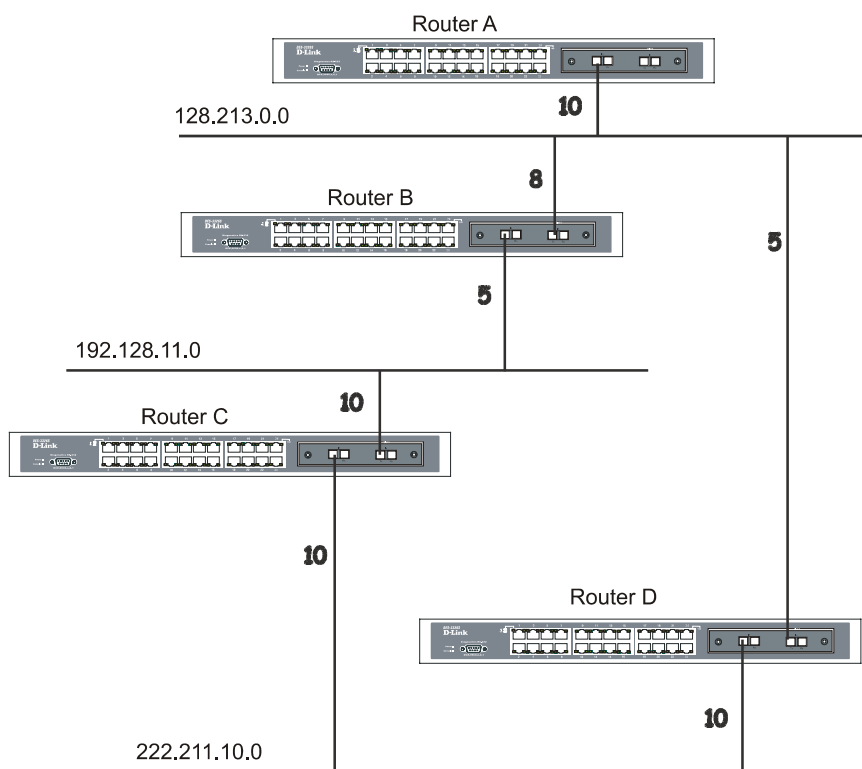
Figure 7- 1. Constructing a Shortest Path Tree
