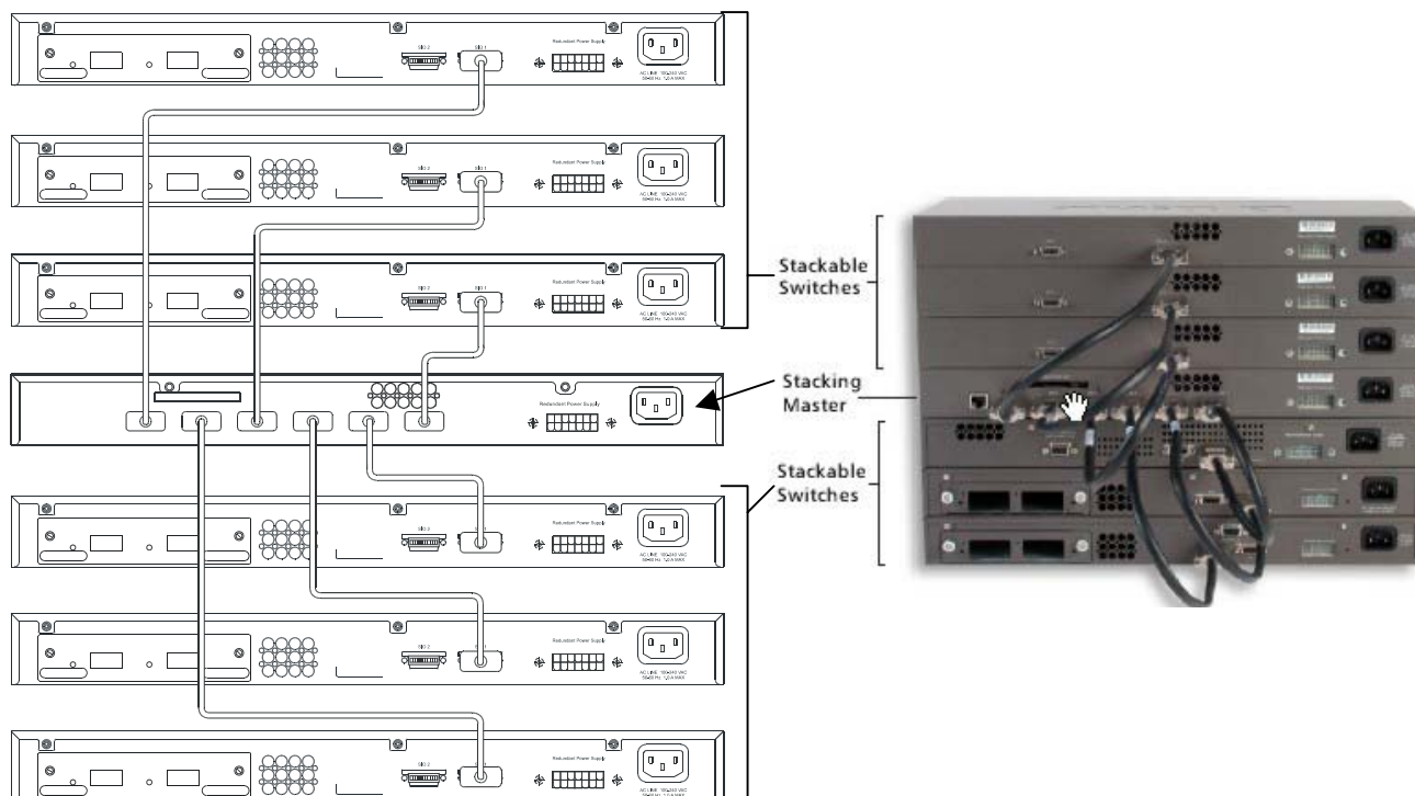
Figure 3- 8. Stacking in a Star Architecture
