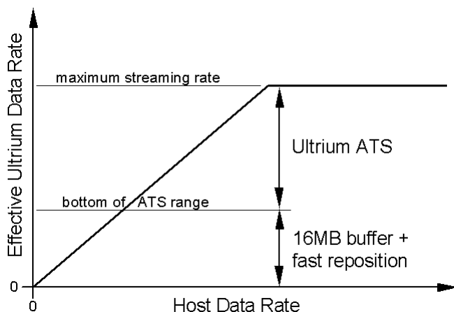
Figure 24: ATS controls effective data rate to match the host data rate
