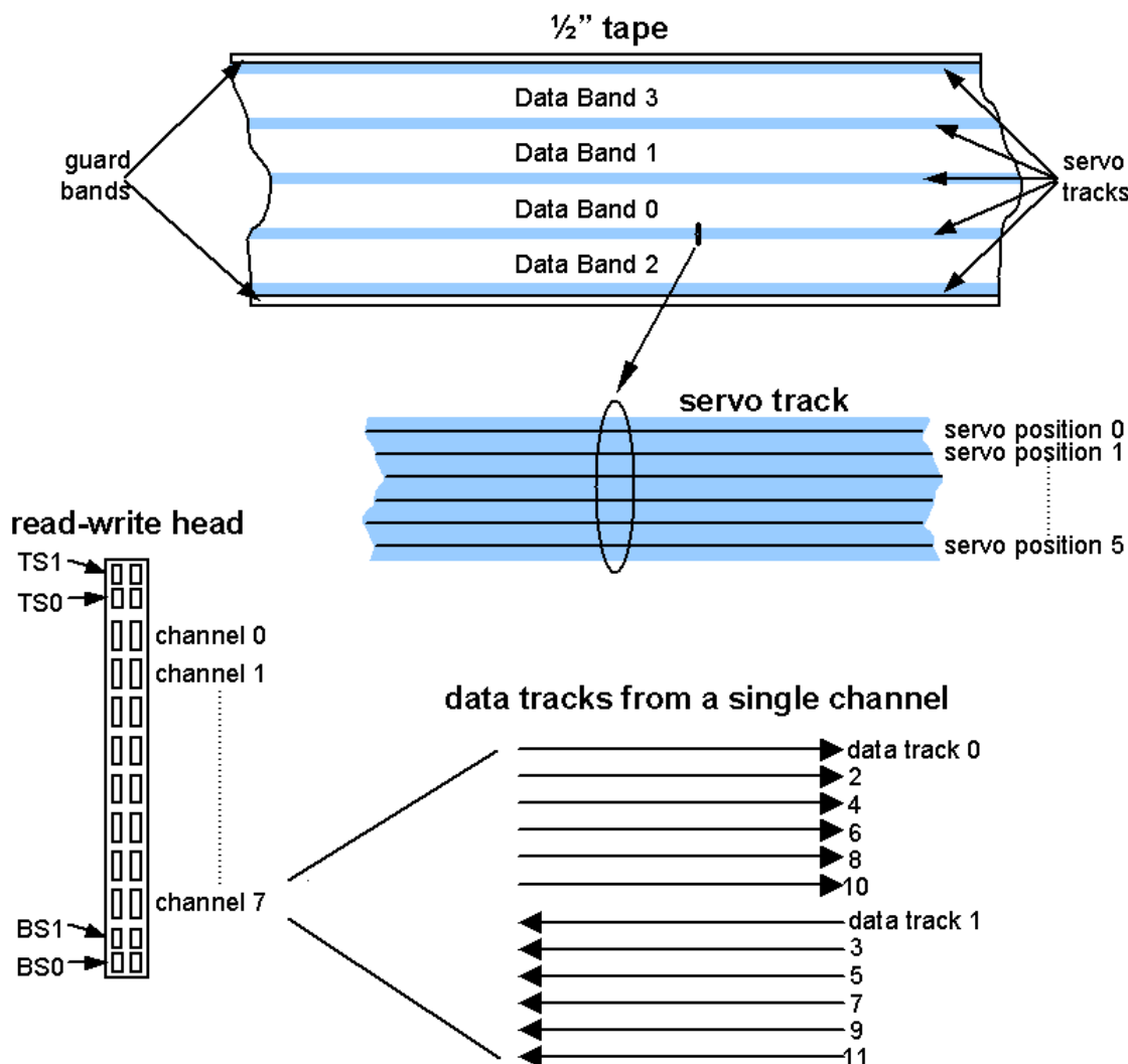
Figure 9: data and servo layout on tape
