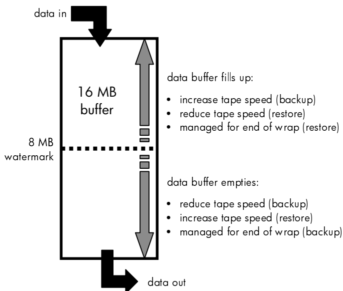
Figure 25: ATS operation
