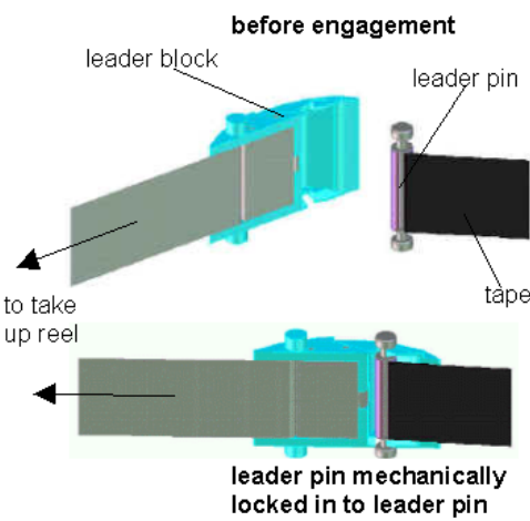
Figure 13: capture and engagement of leader pin into leader block
