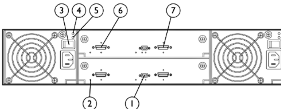
MSA2000 Dual I/O 3.5-inch 12 Drive Enclosure
