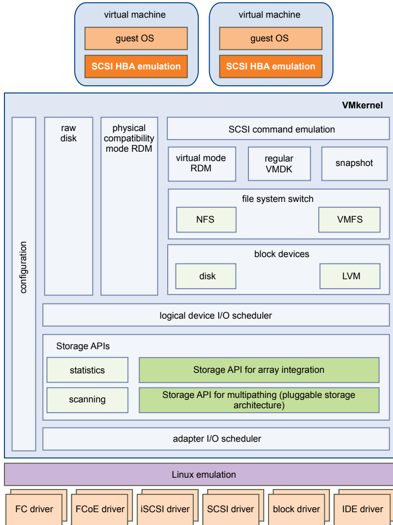
Figure 19-1. VMkernel and Storage
