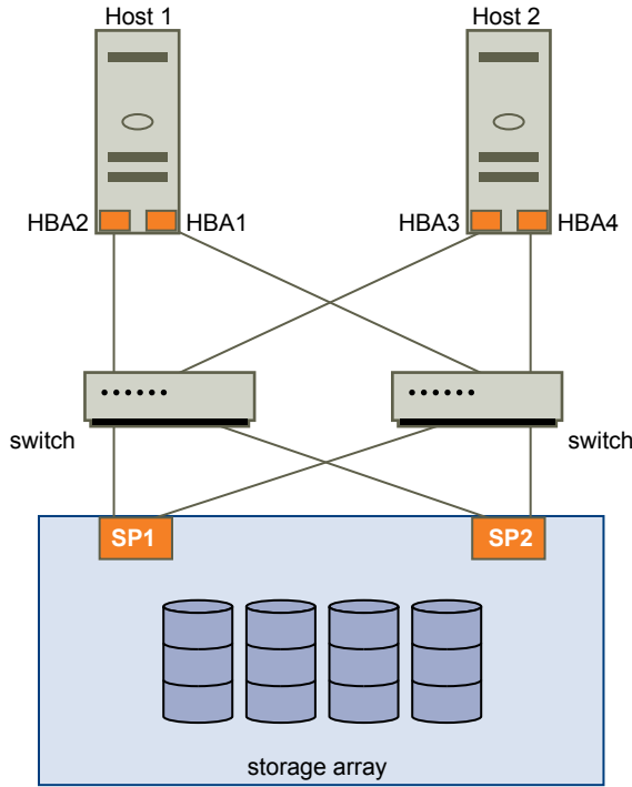
Figure 20-1. Multipathing and Failover with Fibre Channel
